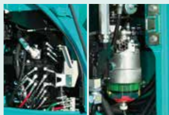
Control valve/water separator tank/air cleaner
